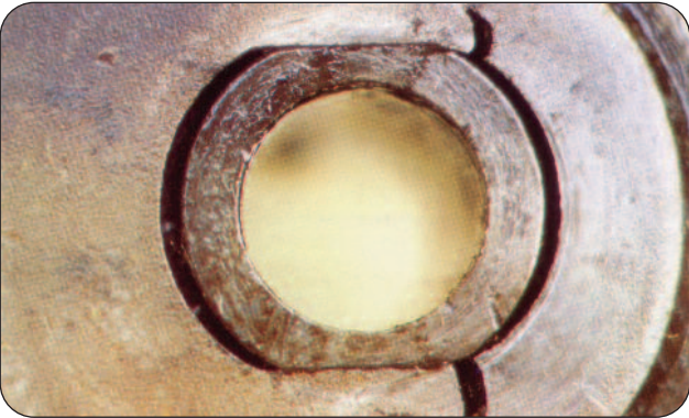
Figure 39 - Mode of Failure - Overload
