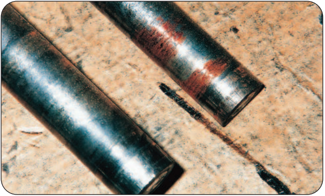
Figure 47 - Mode of Failure - Galling & fretting corrosion
