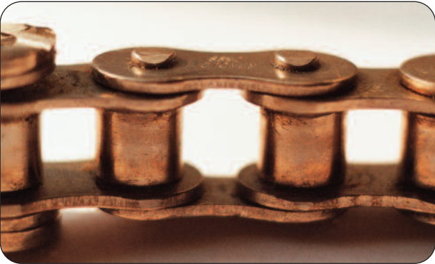
Figure 2 - Mode of Failure - Abrasion
