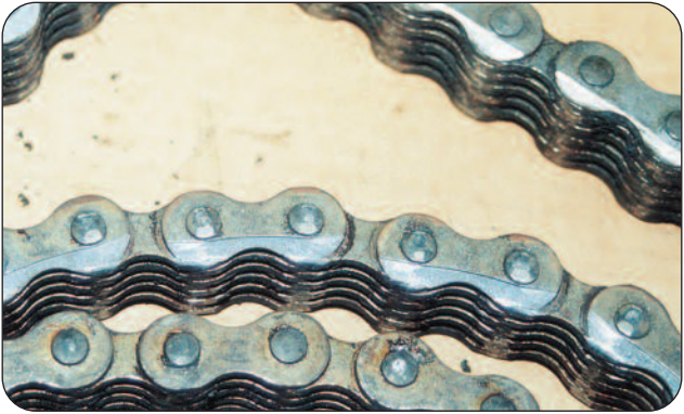
Figure 45 - Mode of Failure - Alignment
