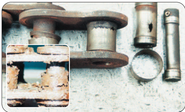
Figure 3 - Mode of Failure - Corrosion
